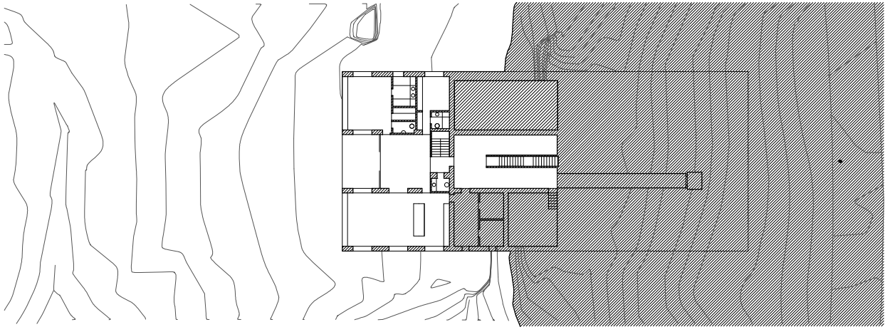
0 1 2m FIRST FLOOR (-3.30)
