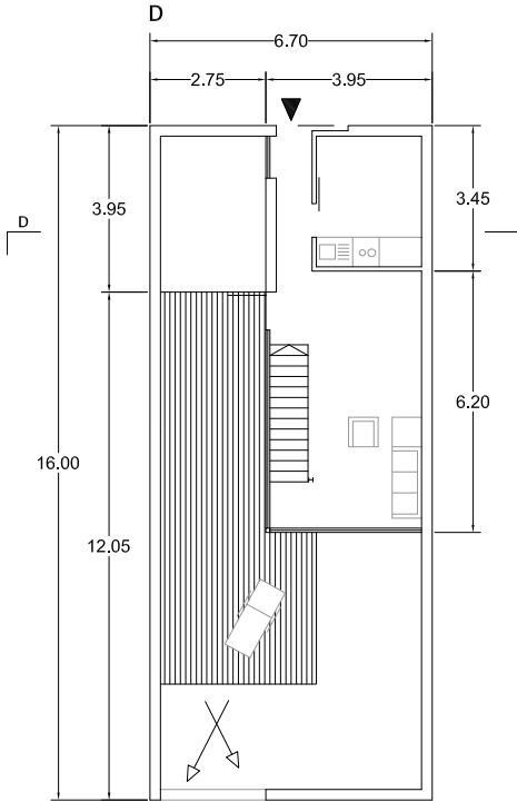
UPPER FLOOR
