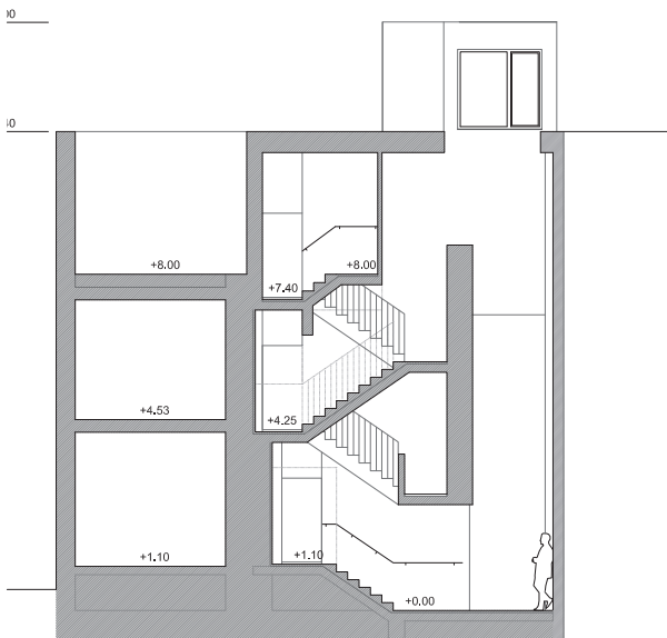
4-4
