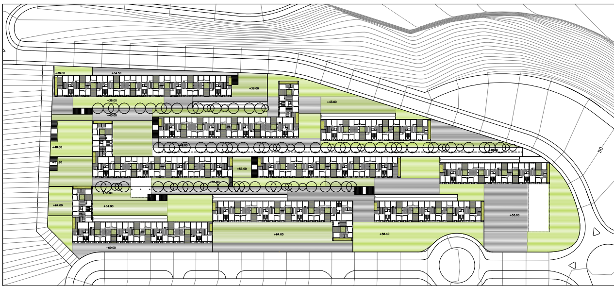
GENERAL PLAN, S:1/1000
