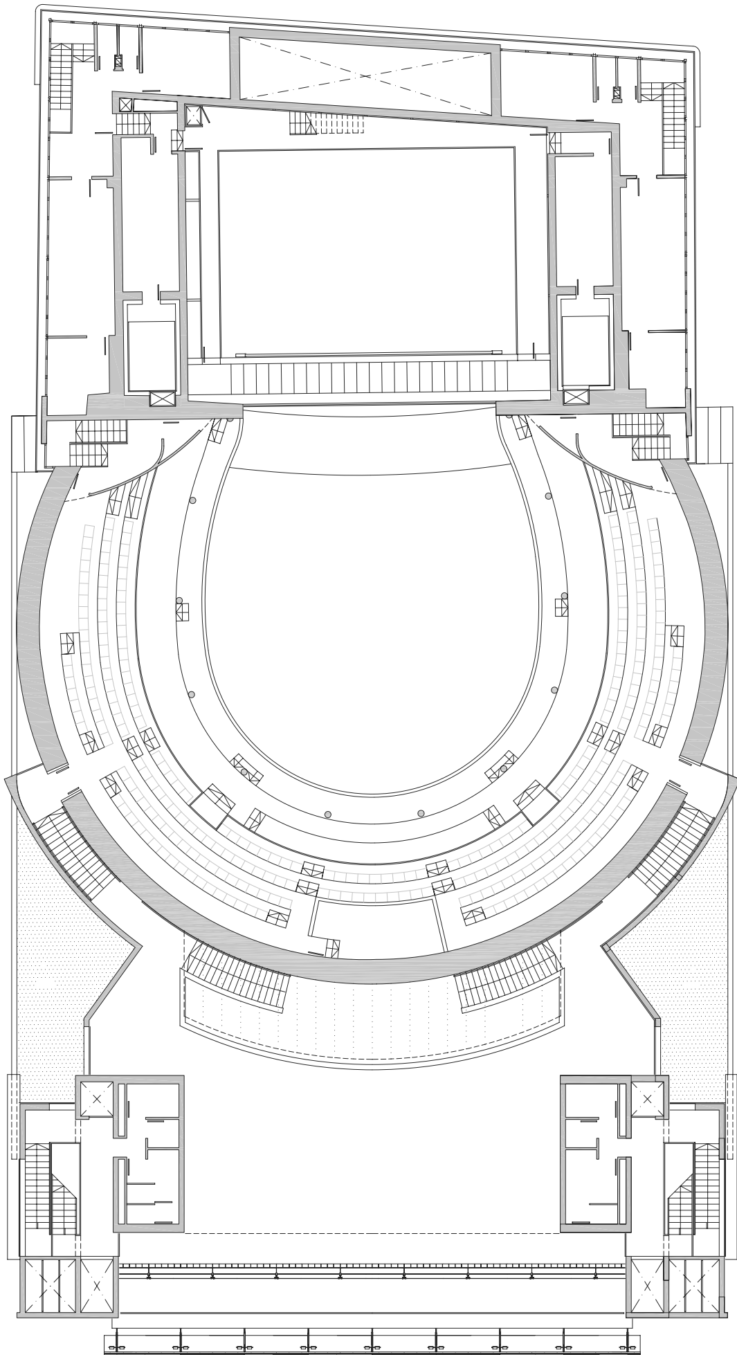
Level 3
