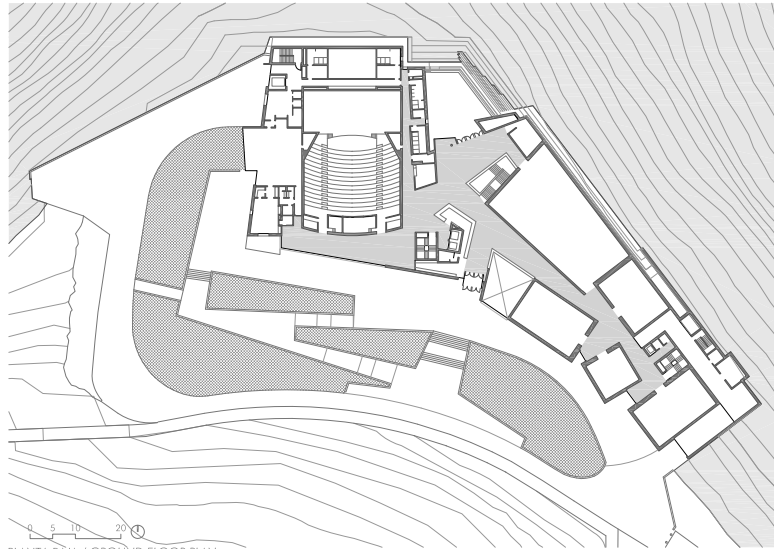
0 5 10 20 PLANTA BAJA / GROUND FLOOR PLAN
