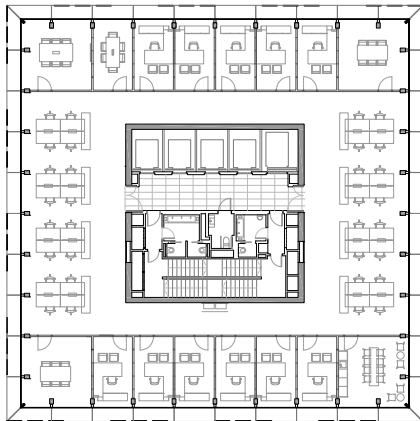
PLANTA TIPO / TYPICAL FLOOR PLAN
