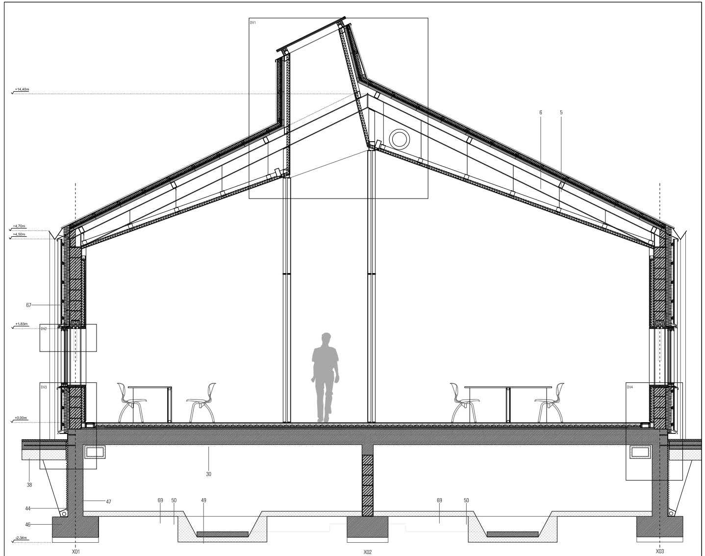
0 1m STRUCTURAL SECTION 03
