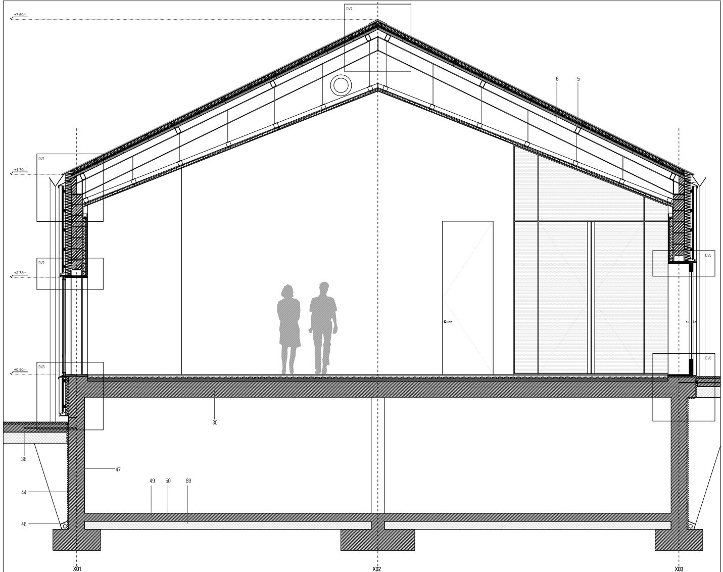
STRUCTURAL SECTION 01
