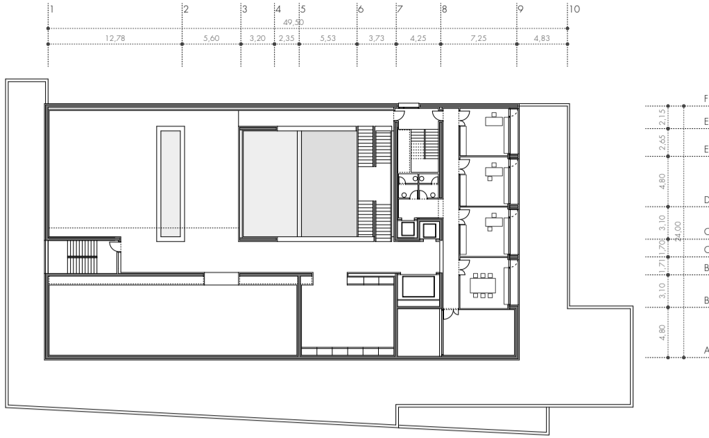
PLANTA TERCERA. SALAS. CONSERVADORES cota +11,56 LEVEL 3. EXHIBITION ROOMS. CURATORS
