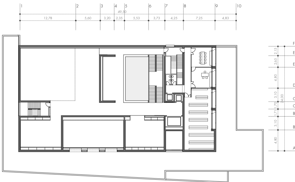
PLANTA PRIMERA. SALAS. BIBLIOTECA cota +4,08 LEVEL 1. EXHIBITION ROOMS. LIBRARY
